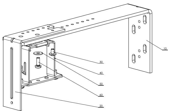
Support réglable double – fixe 306 – 368 mm P 010/47 (2-01805-0000)
